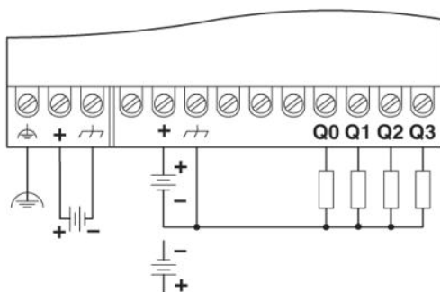
Connection diagram
